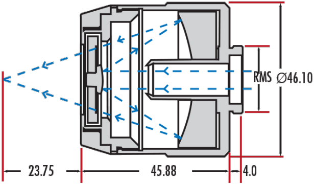
20X ReflX™ Objectives
