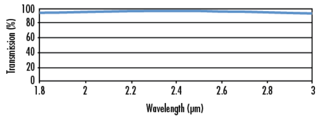
1.8 - 3 \mu m AR Coating
