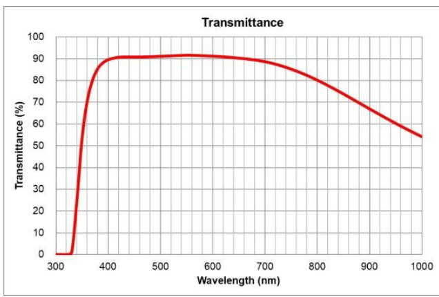
LUCPLFN60X2 Transmission Graph
