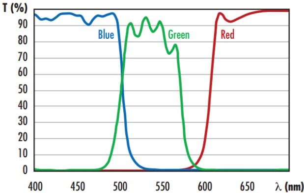
Additive Filters Typical Transmittance Curves
